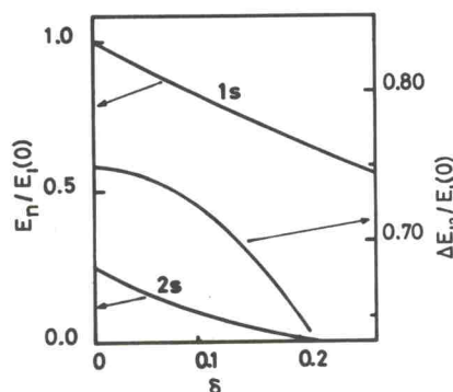
Fig. 6. The variation in the binding energy, E_n , of an n^{\text{th}} order exciton with the screening parameter \delta (after Harris[25]).
